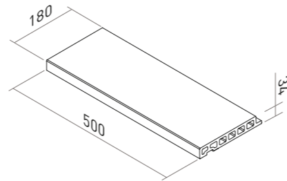
CANARIAS EDGE BORDE CANARIAS Ref. BSCA 0000 18x50 (M-729) pz MONOBLOCK
