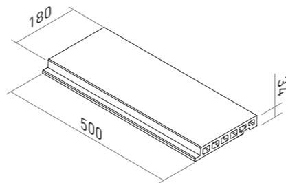
GRATE SUPPORT SOPORTE P/REJILLA Ref. BSCA 0000 18x50 (M-729) pz MONOBLOCK
